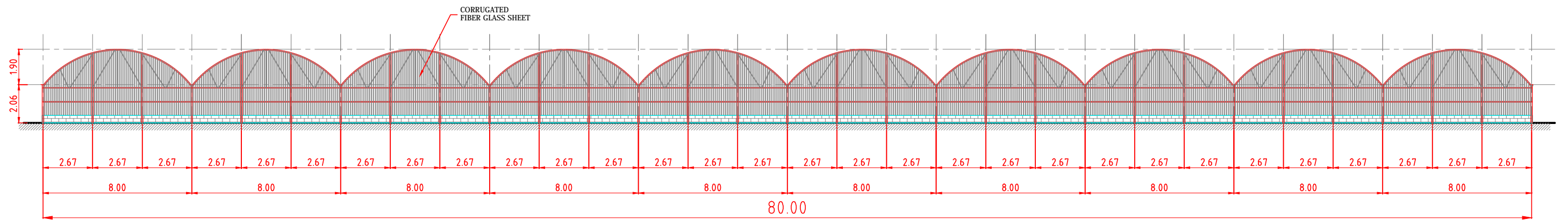
TYPICAL REAR VIEW ELEVATION
